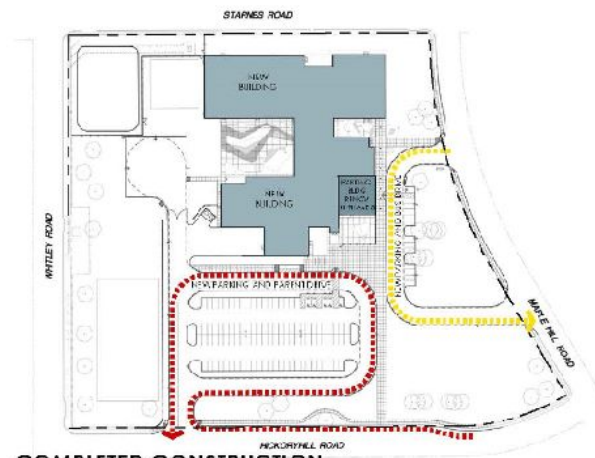
COMPLETED CONSTRUCTION
